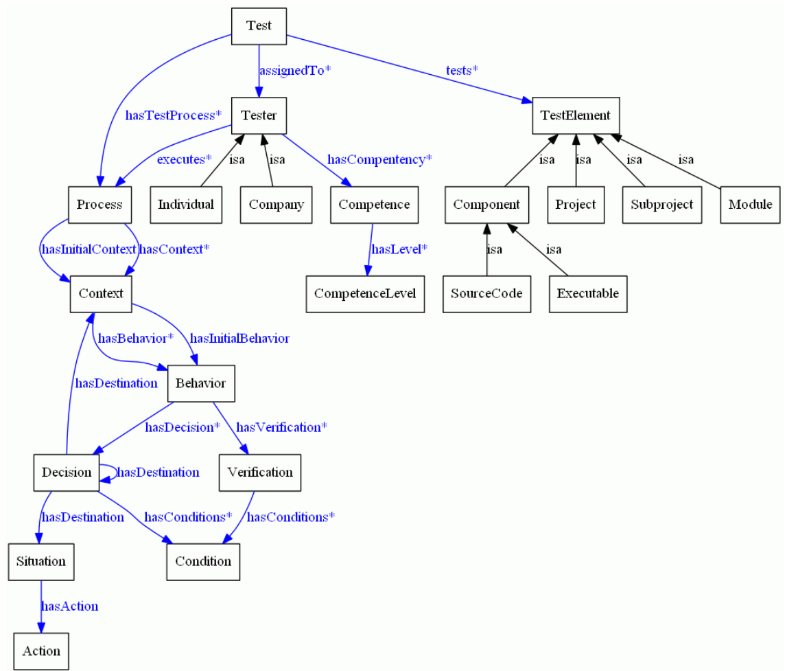
Fig. 1. . SABUMO-dTest ontology (partial view)
