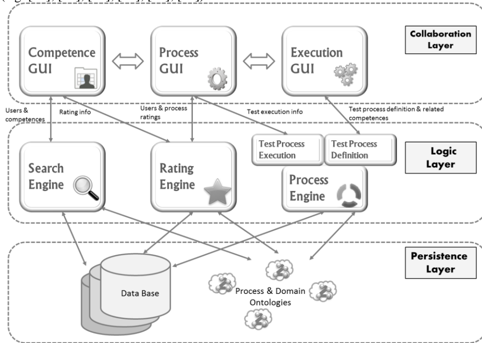
Fig. 2. . SABUMO-dTest architecture
